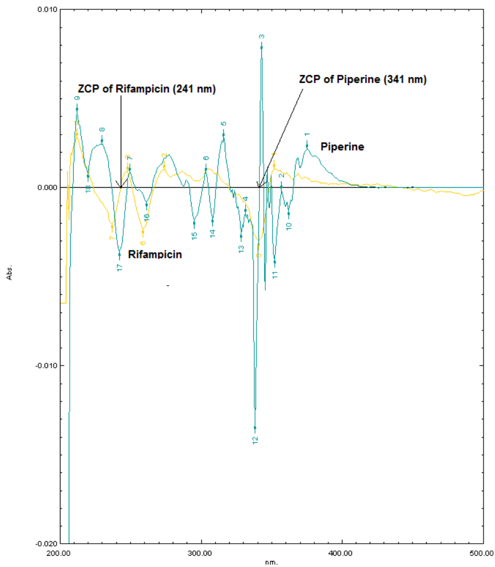
Figure 4: Overlain Second order Derivative absorption spectra of RIFA and PIPE in methanol
