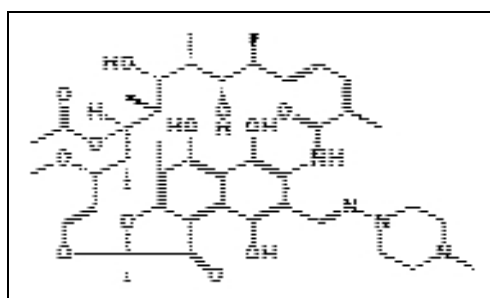
Figure 2: Structure of Rifampicin
