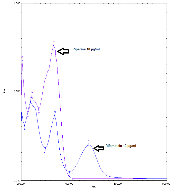
Figure 3: Overlain zero-order absorption spectra of RIFA and PIPE in methanol
