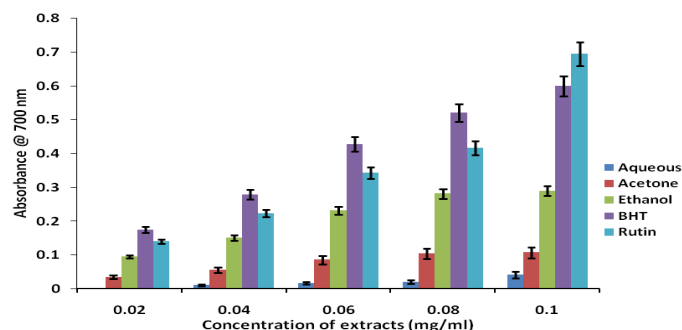
Figure 2 Ferric reducing power determinations for the alcoholic & aqueous extract of C. macrophylla (data are presented as means \pm standard deviation of three replicate with significant increases from all samples tested.)
